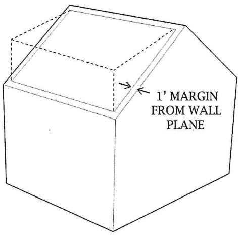
Gable roof
